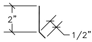
ANGLE CLEAT
