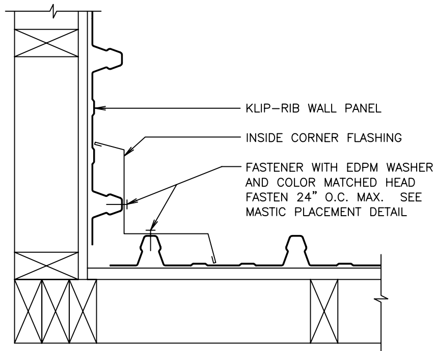
INSIDE CORNER
