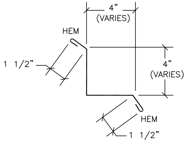
INSIDE CORNER
